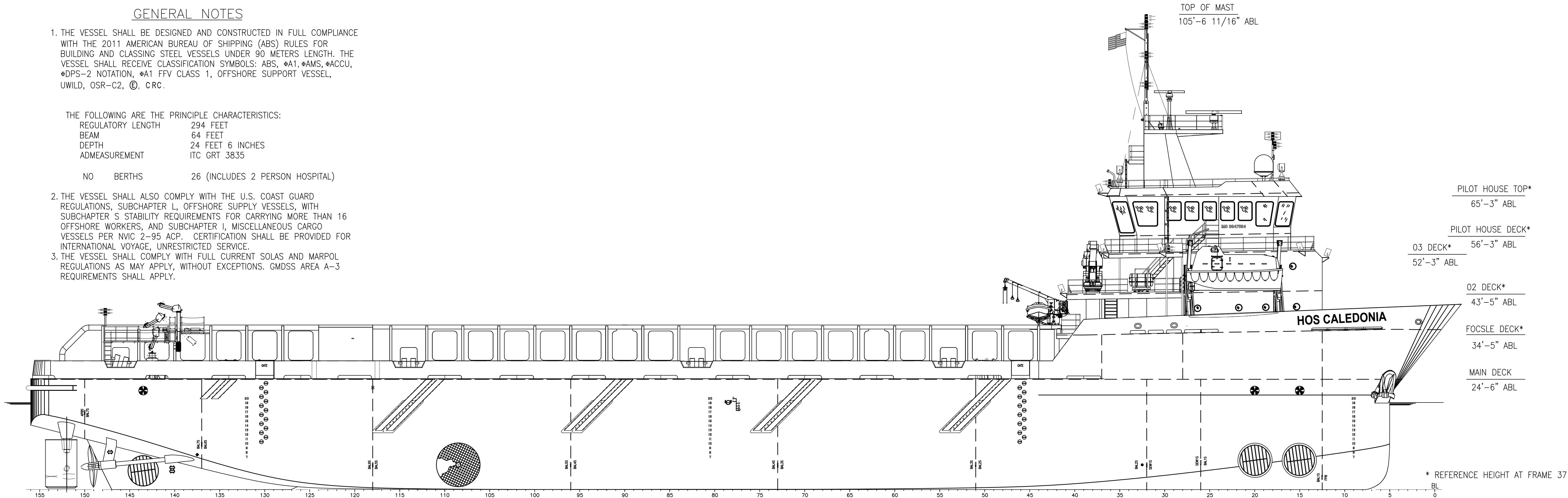
OUTBOARD PROFILE
