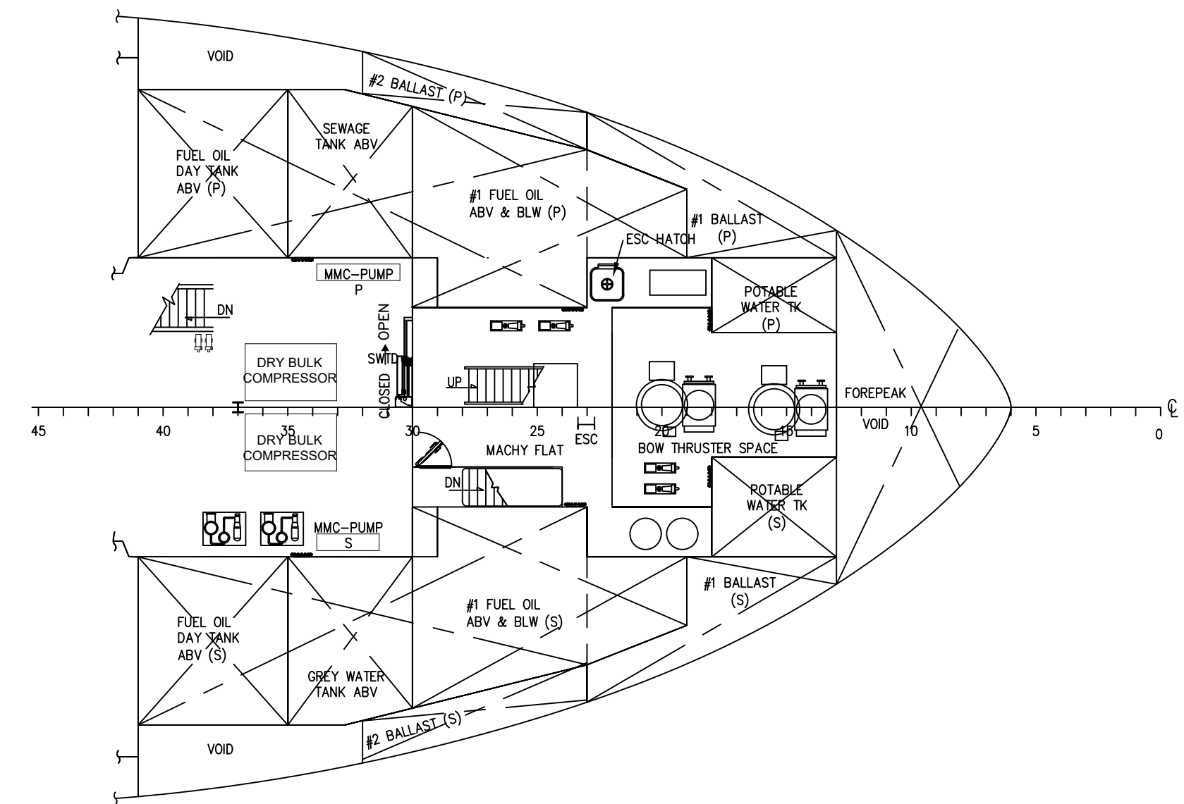
MEZZANINE FLAT
