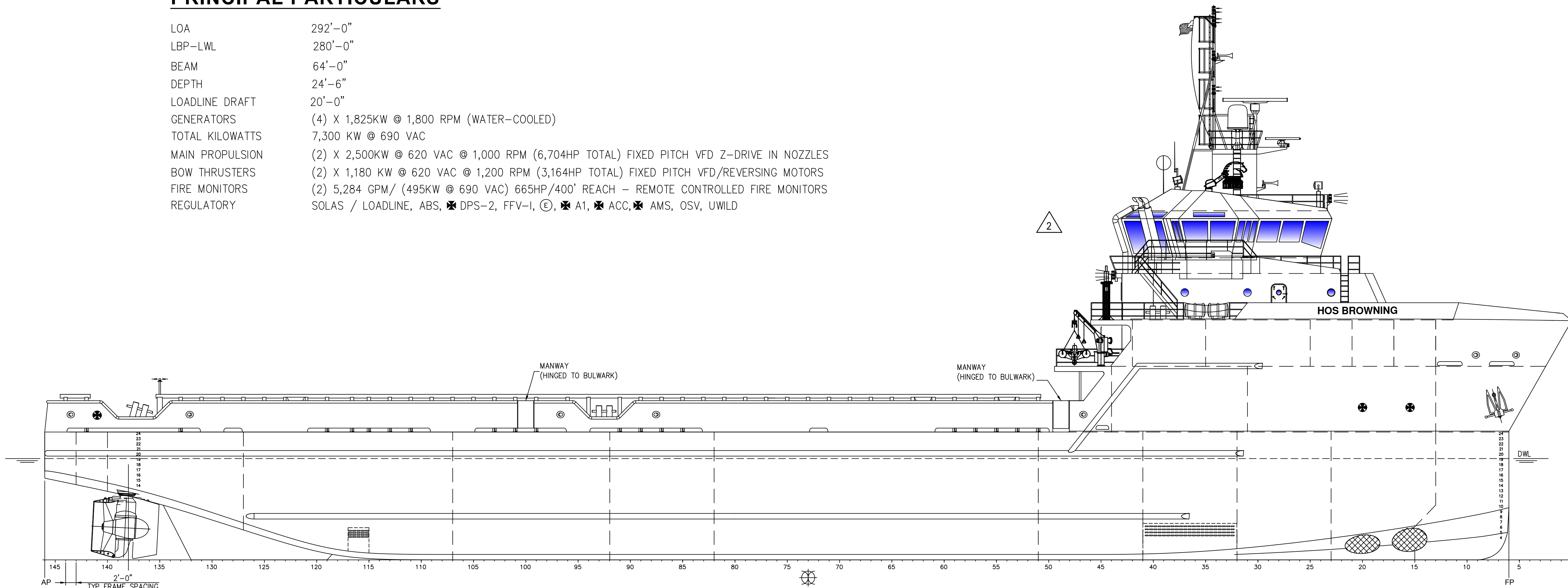
OUTBOARD PROFILE
