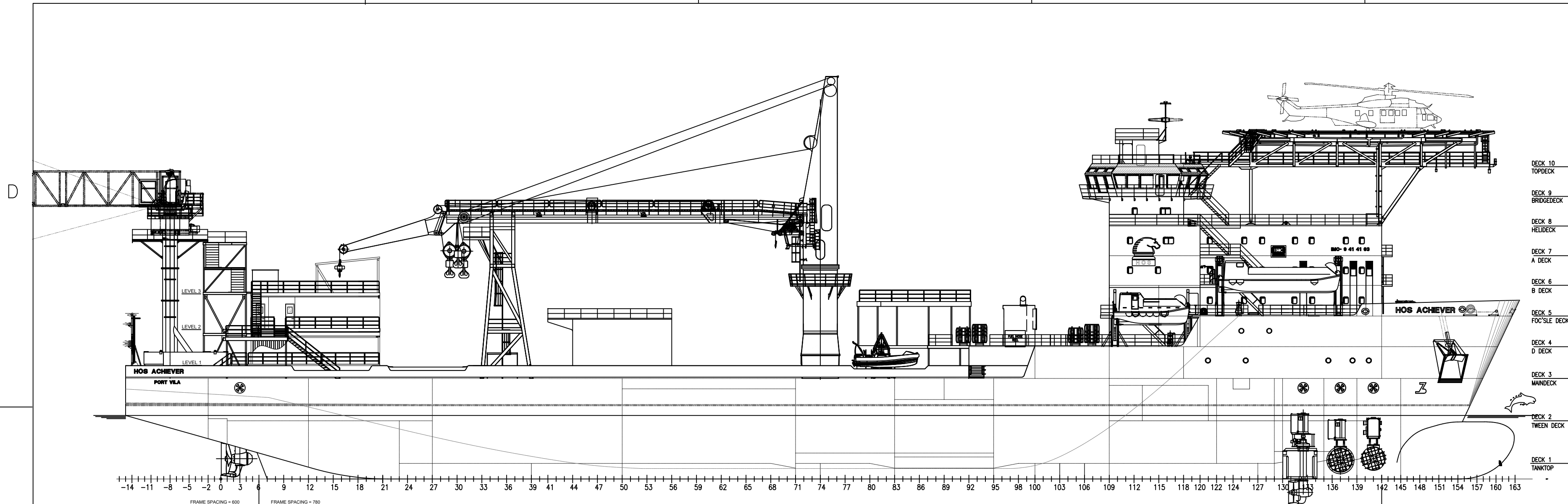
OUTBOARD PROFILE STBD SIDE SCALE: 1:300
